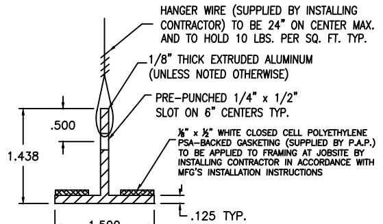
TEE DETAIL
